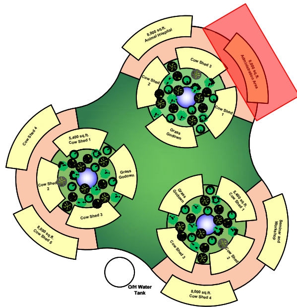
KEY PLAN OF ADMIN BLOCK
